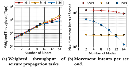
Figure 9: Application level metrics on SCALO.
