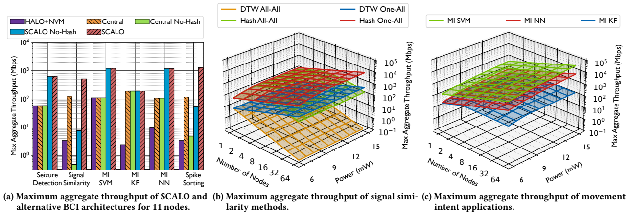
Figure 8: Experimental quantification of SCALO's benefits.
