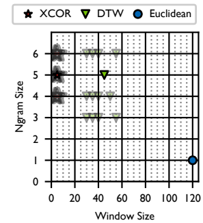
Figure 14: Hash flexibility.
