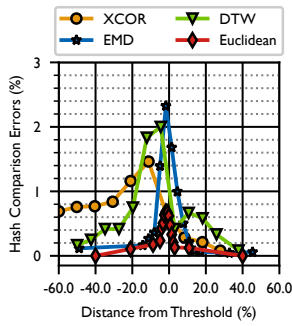
Figure 11: Hash errors.
