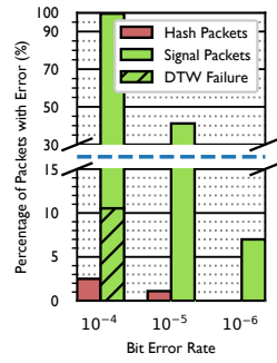
Figure 12: Network errors.
