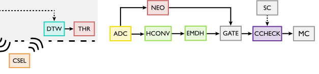
Figure 5: Seizure detection and propagation on SCALO. The colors of the PEs are matched with the high-level tasks from Figure 3a.
